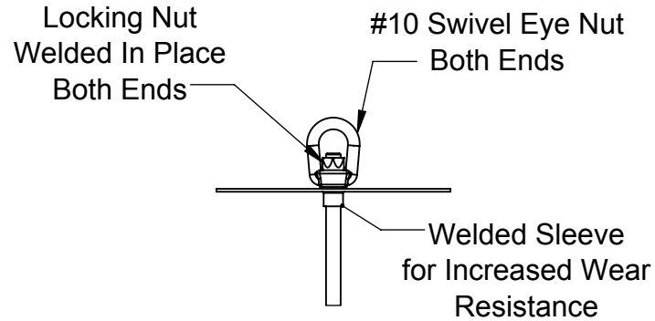
DETAIL A SCALE 1 : 15
